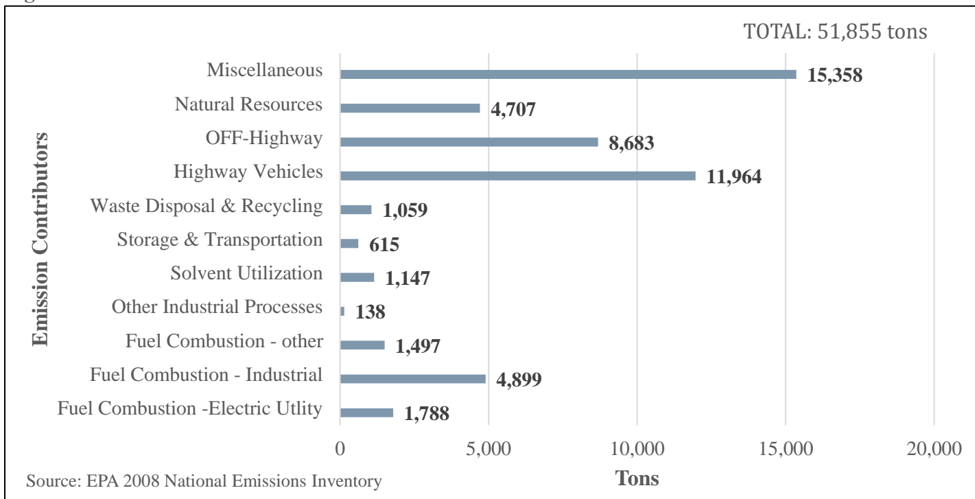
Figure 3. Emissions Contributors 2008
